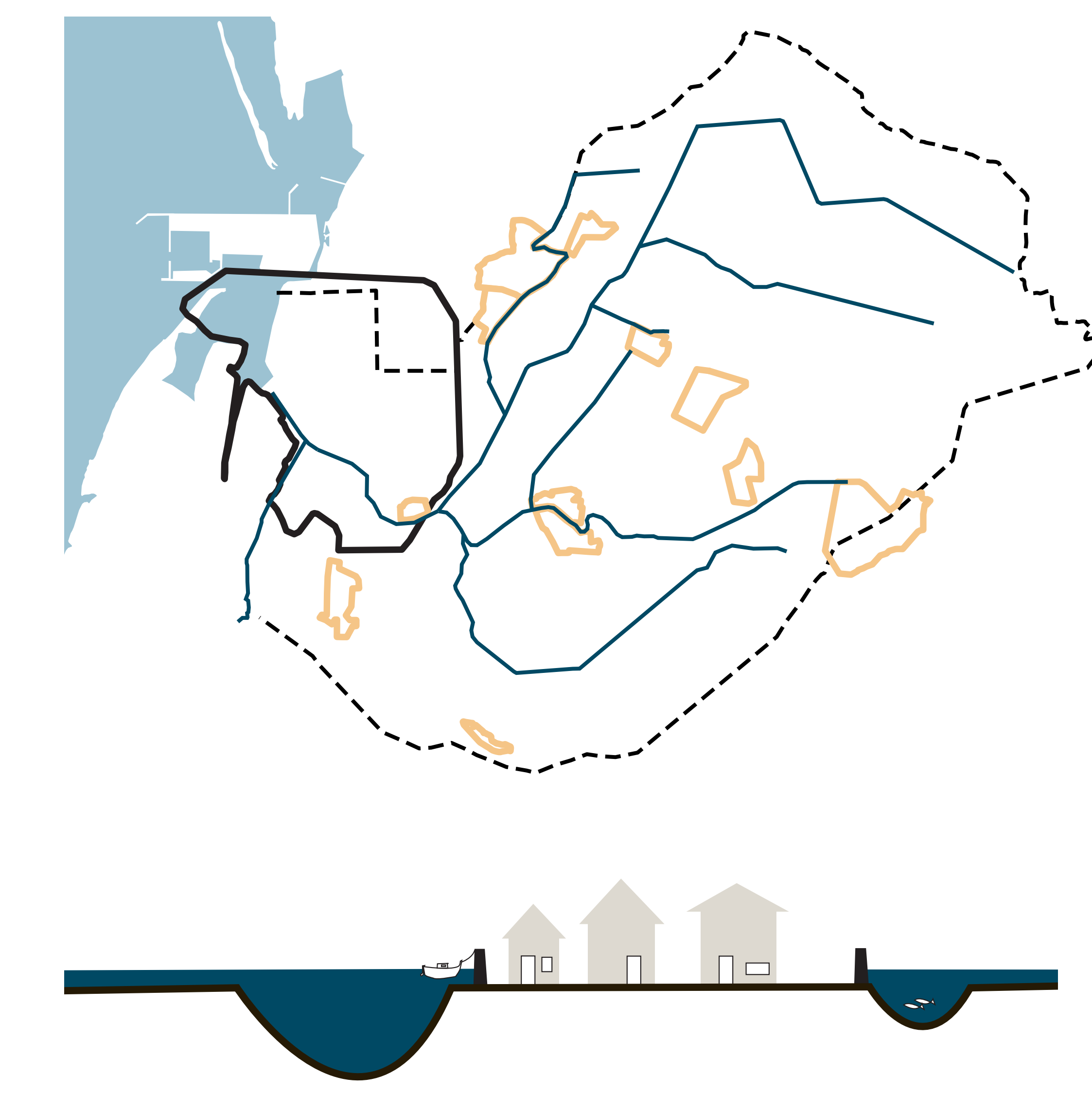
C: village floodproof 村落防洪
